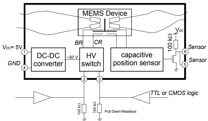
Electrical Schematic Diagram
