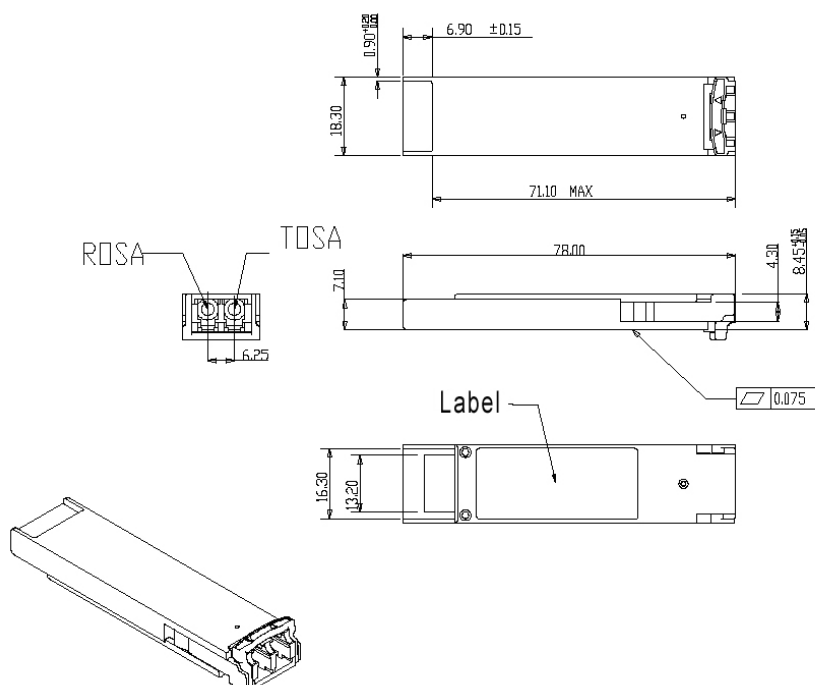
Figure3. Mechanical Specifications
