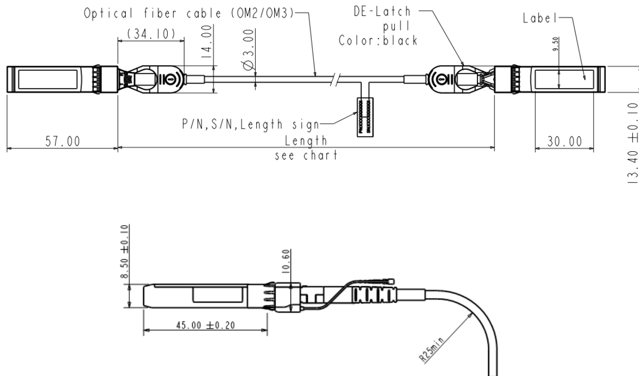
Figure1. Mechanical Specifications
