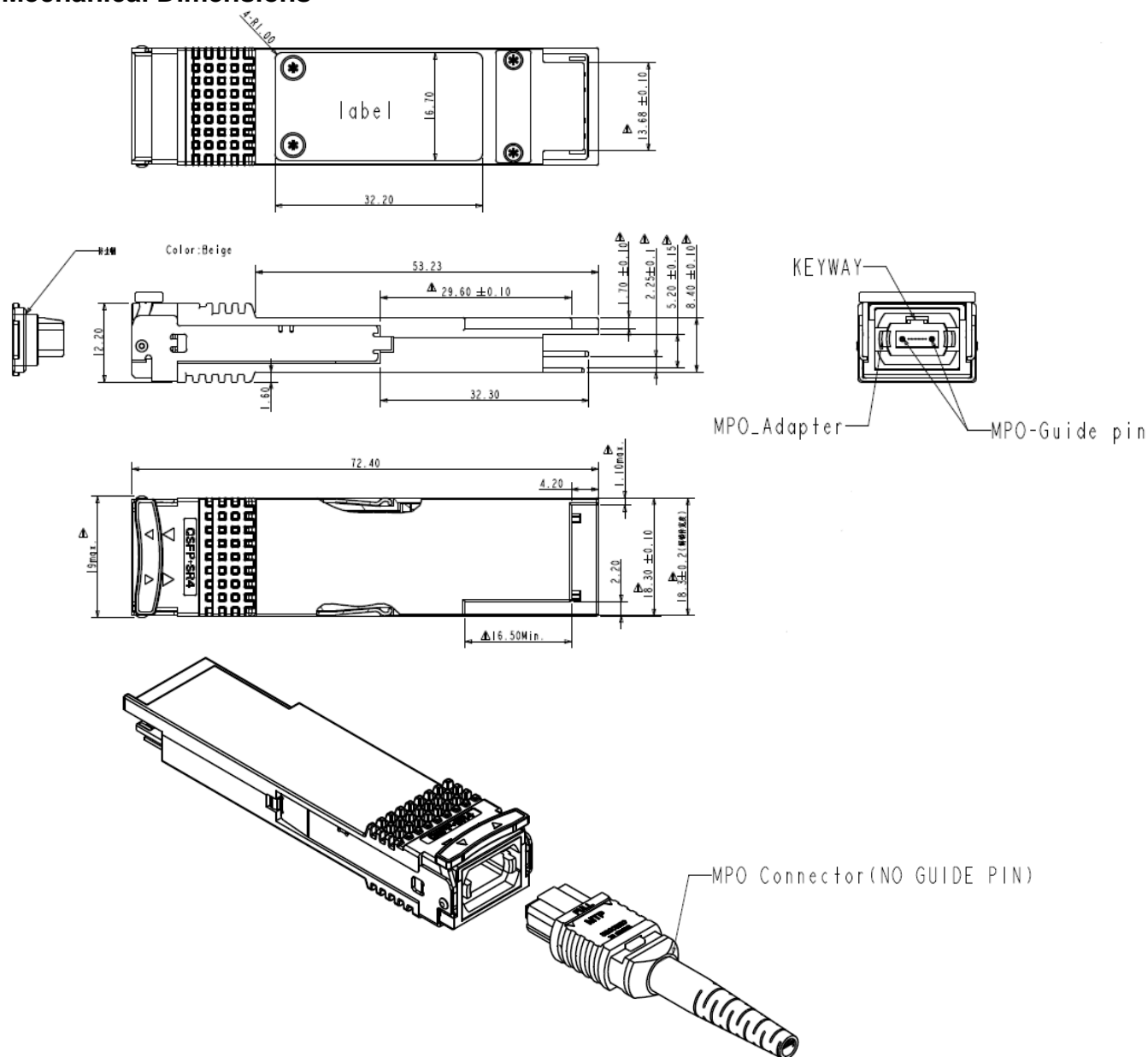
Figure10. Mechanical Specifications
