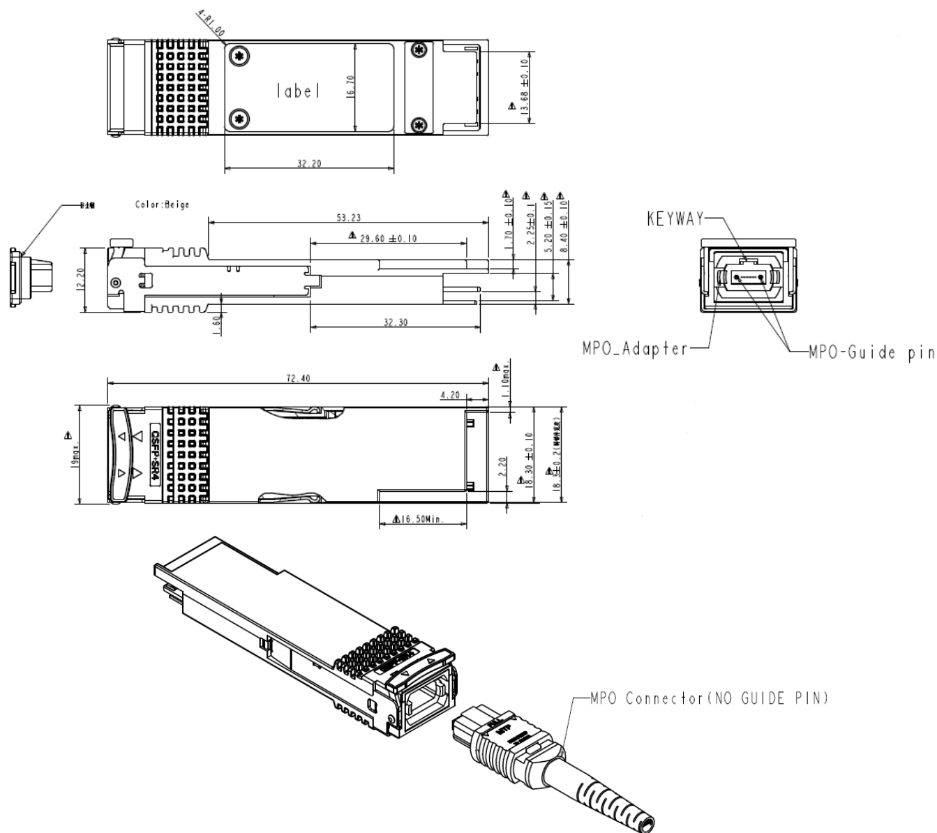
Figure10. Mechanical Specifications
