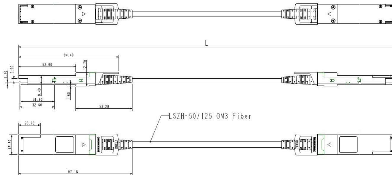
Figure9. Mechanical Specifications
