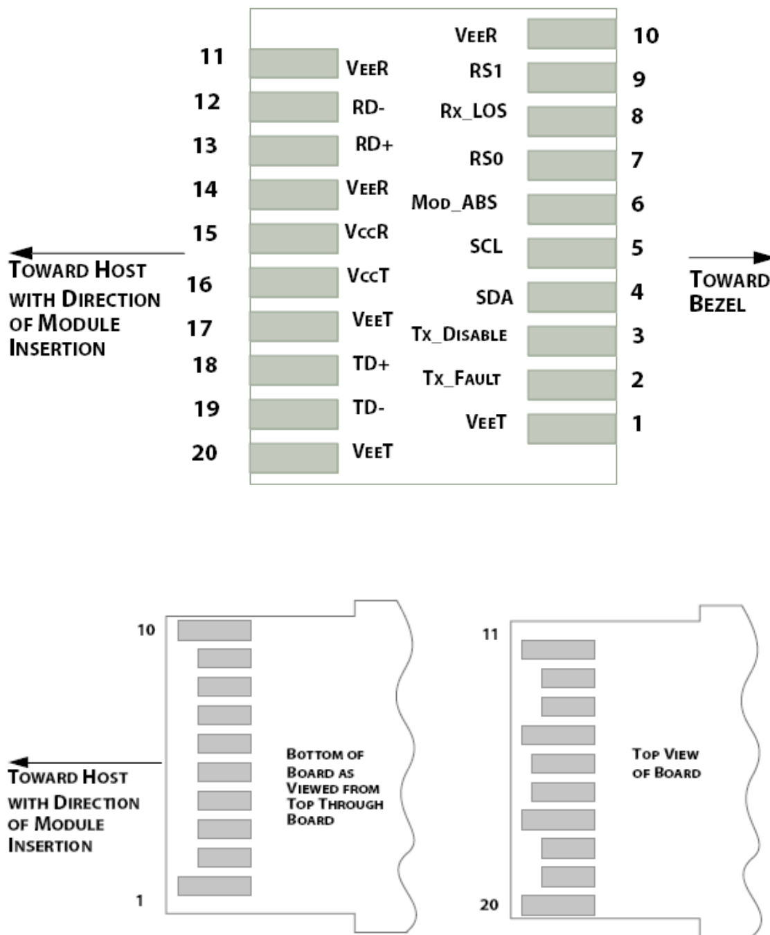
Figure2.Electrical Pin-out Details
