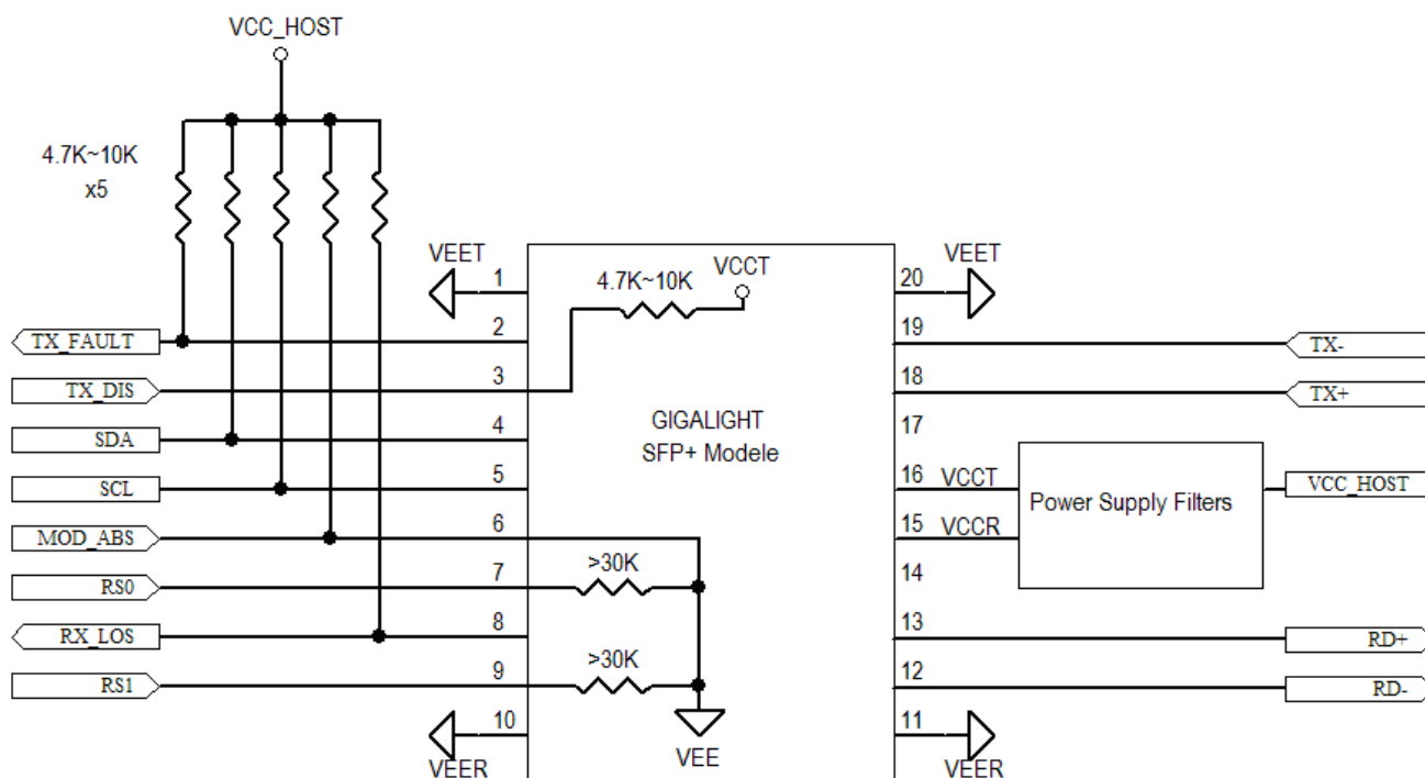
Figure5. Host-Module Interface
