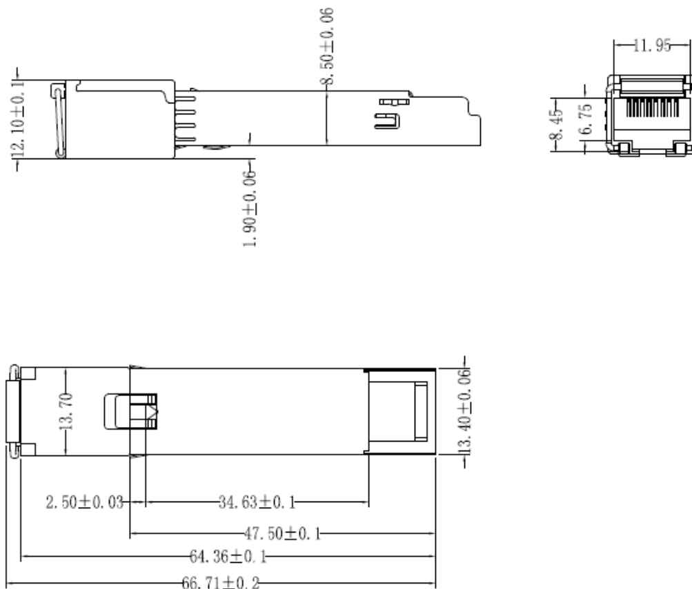
Figure 2. Mechanical dimensions
