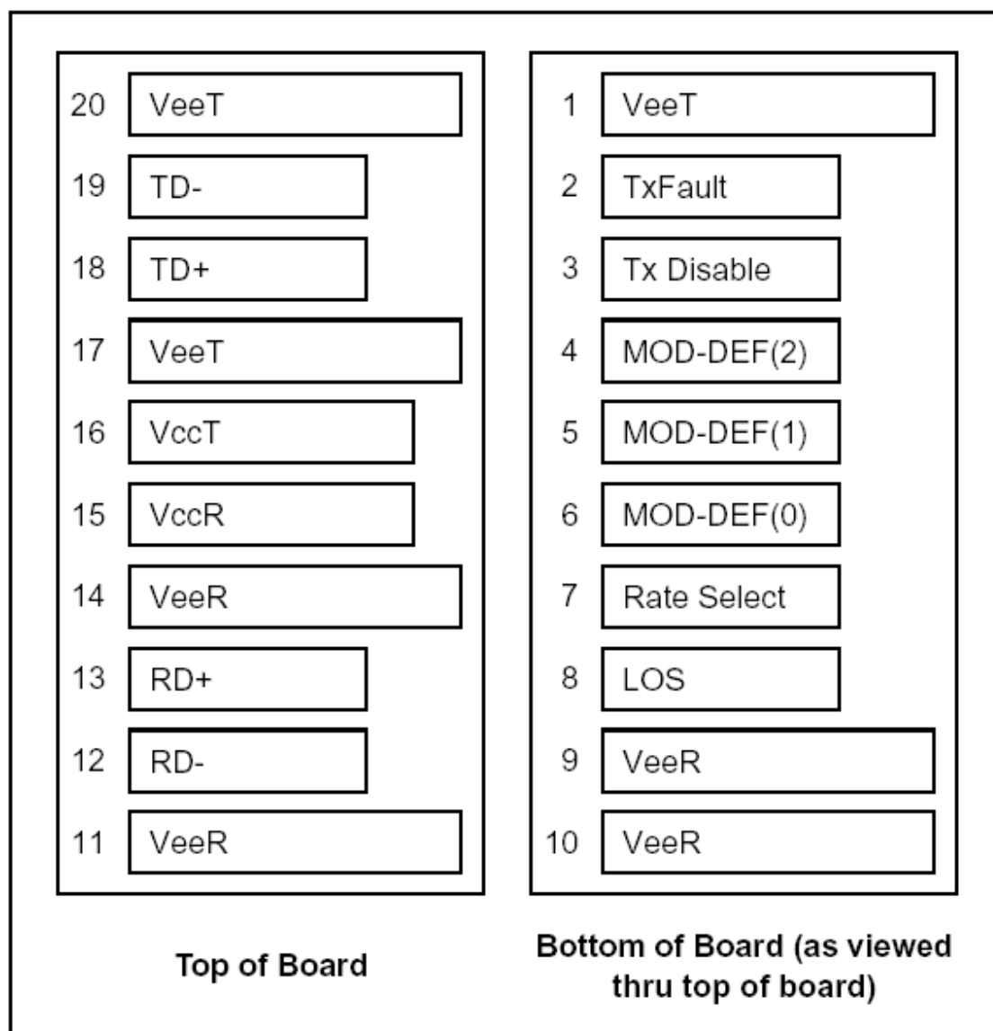
Figure 1. Pin Definitions
