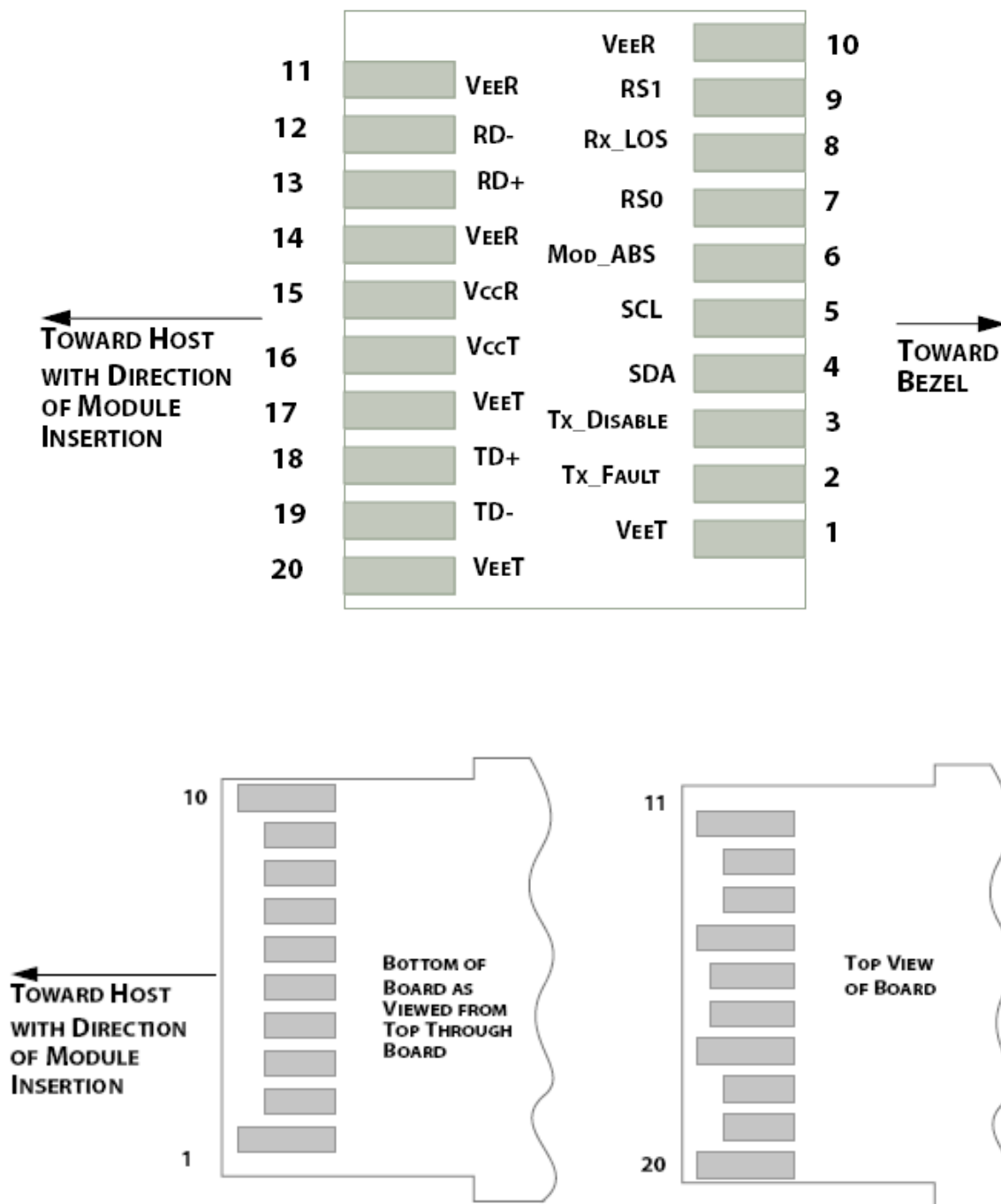
Figure2.Electrical Pin-out Details
