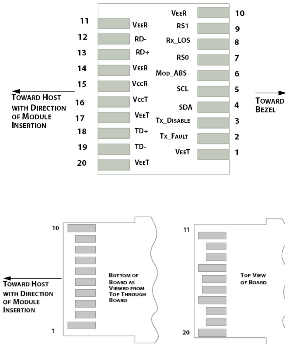
Figure2.Electrical Pin-out Details
