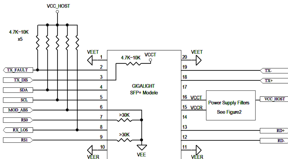
Figure3. Host-Module Interface
