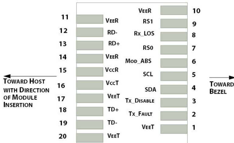
Figure1.Electrical Pin-out Details
