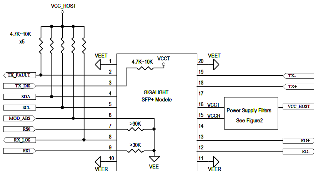
Figure3. Host-Module Interface
