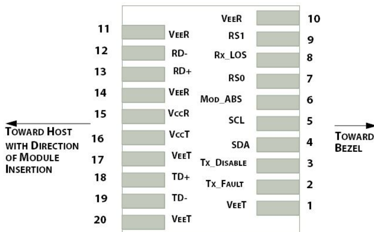
Figure1.Electrical Pin-out Details
