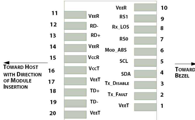
Figure1.Electrical Pin-out Details
