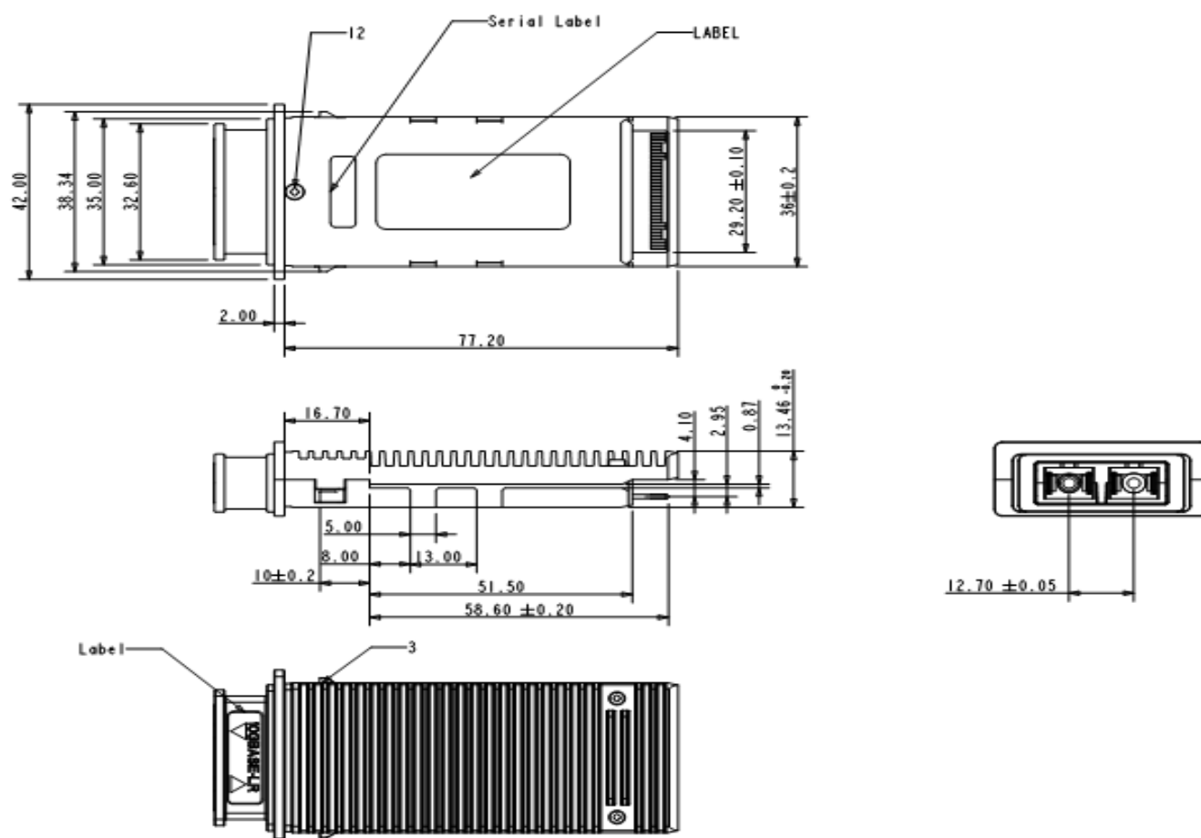
Figure3. Mechanical Dimensions
