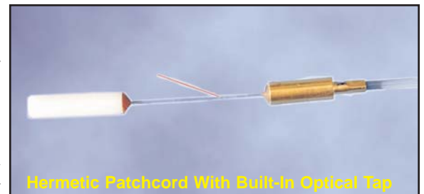
Hermetically sealable patchcords with glass solder and 1.4mm OD circular Zirconia ferrule (puck)
