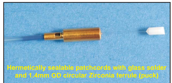
16 Channel Hermetically sealable ribbon fiber patchcords with glass solder
