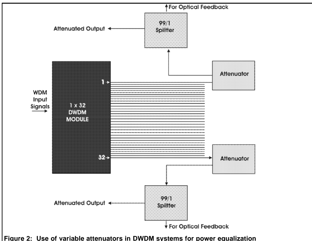
Figure 2: Use of variable attenuators in DWDM systems for power equalization
