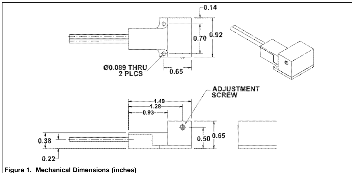
Figure 1. Mechanical Dimensions (inches)
