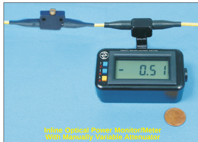
Inline Optical Power Monitor/Meter With Digital Display
