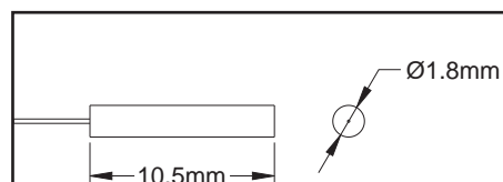
Figure 10: 1.8mm Ceramic Ferrule
