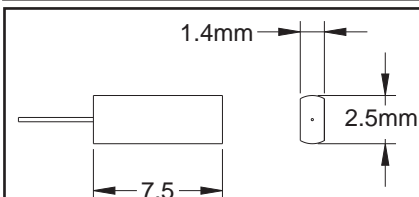
Figure 13: Rectangular Glass Ferrule
